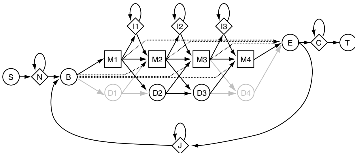
Figure 2.1: The Plan7 architecture. Squares indicate match states (modeling consensus positions in the alignment). Diamonds indicate insert states (modeling insertions relative to consensus) and special random sequence emitting states. Circles indicate delete states (modeling deletions relative to consensus) and special begin/end states. Arrows indicate state transitions. See text for more details.
